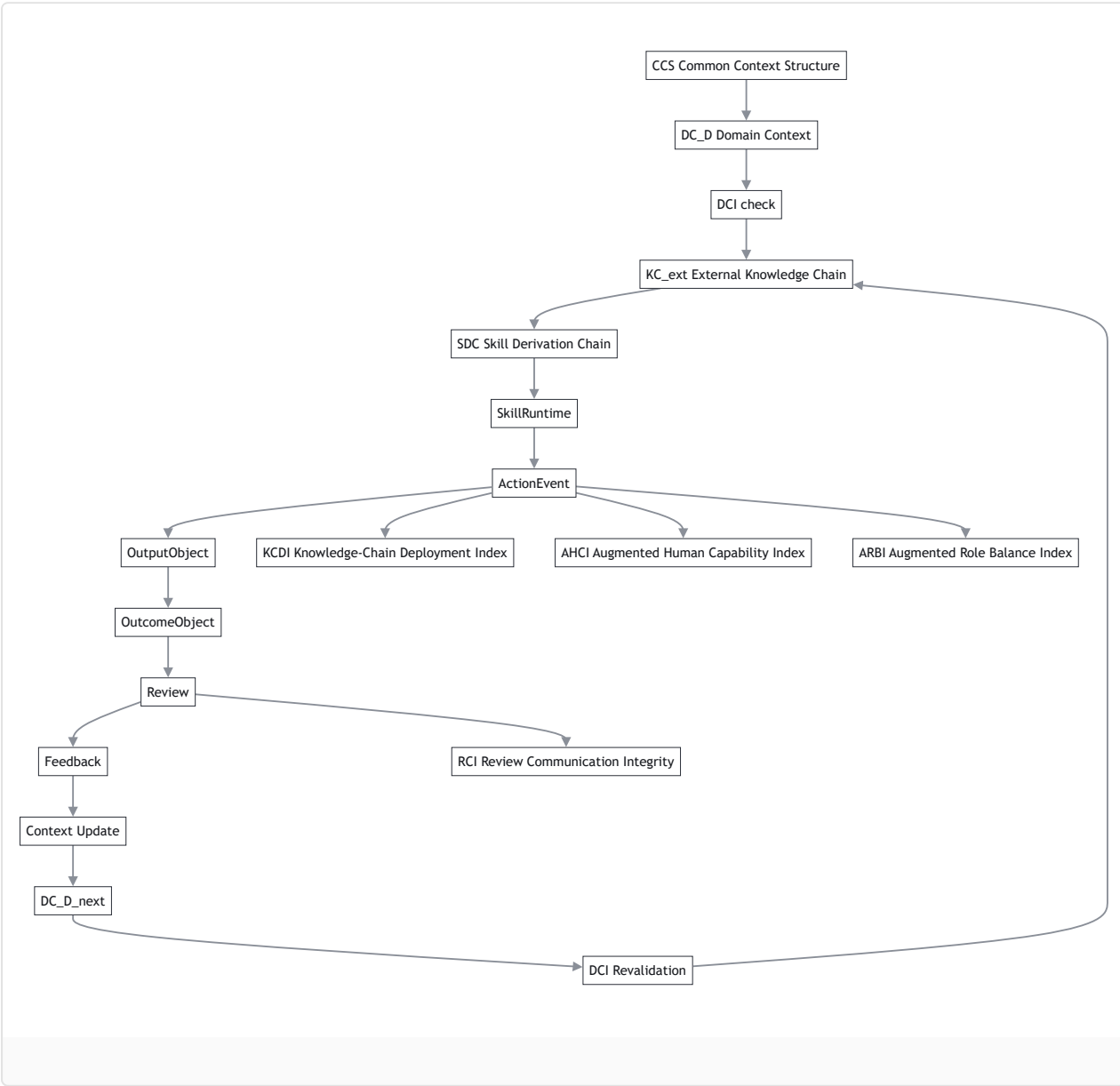
Figure 4. KAC with operational metrics — KCDI, AHCI, and ARBI branch from ActionEvent, and RCI from Review, to measure execution and observation.
